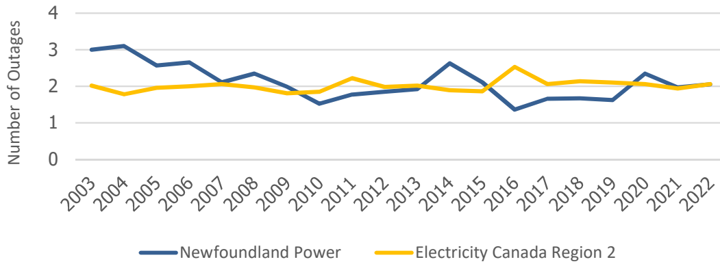
Figure 2 Newfoundland Power vs. Canadian Average SAIFI - Normal Operating Conditions (2003-2022)
