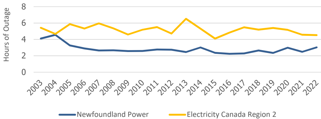
Figure 1 Newfoundland Power vs. Canadian Average SAIDI - Normal Operating Conditions (2003-2022)
