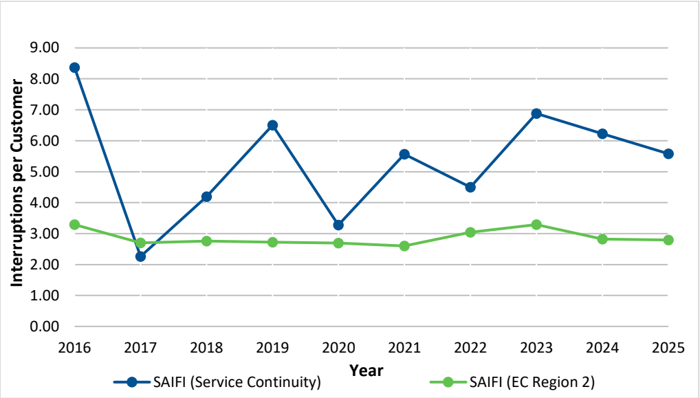
Chart 5: SAIFI Excluding Major Events – Northern
