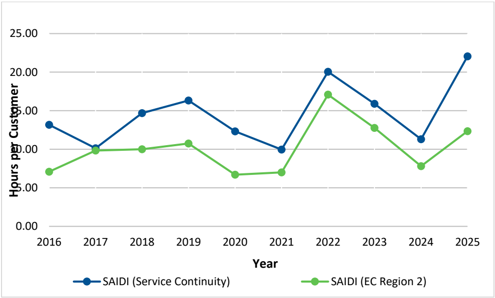
Chart 8: SAIDI Including Major Events – Northern
