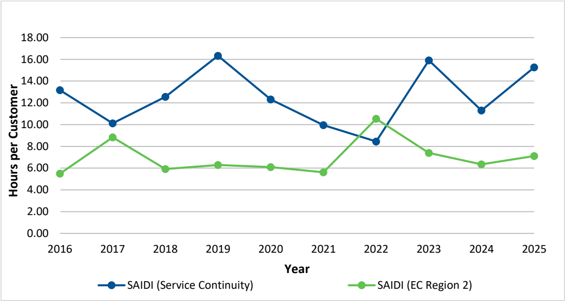
Chart 7: SAIDI Excluding Major Events – Northern
