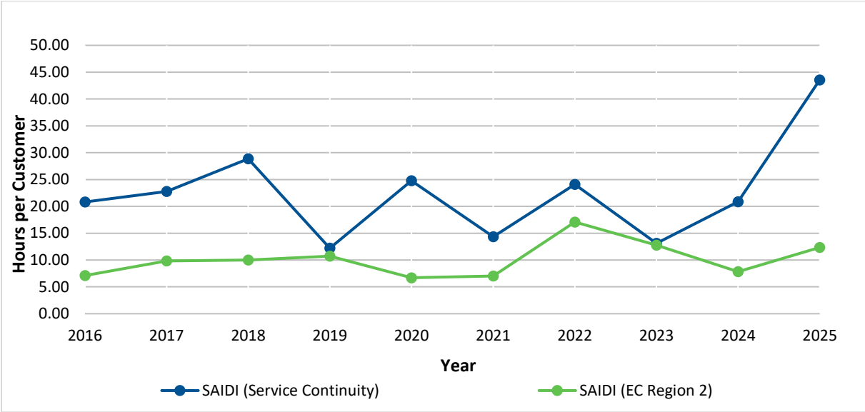
Chart 4: SAIDI Including Major Events – Central
