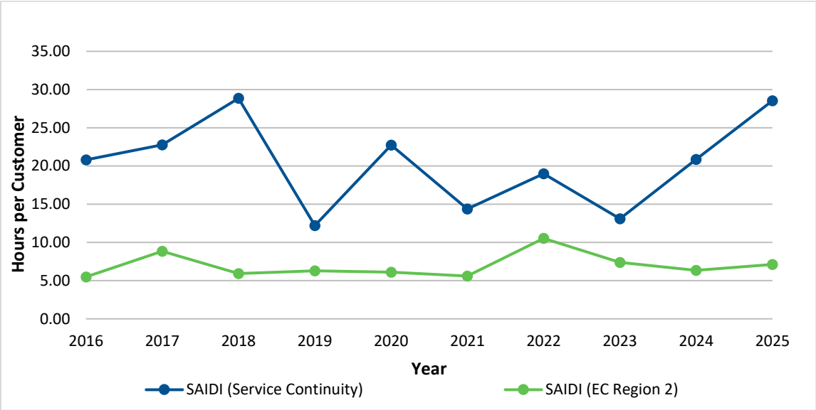
Chart 3: SAIDI Excluding Major Events – Central
