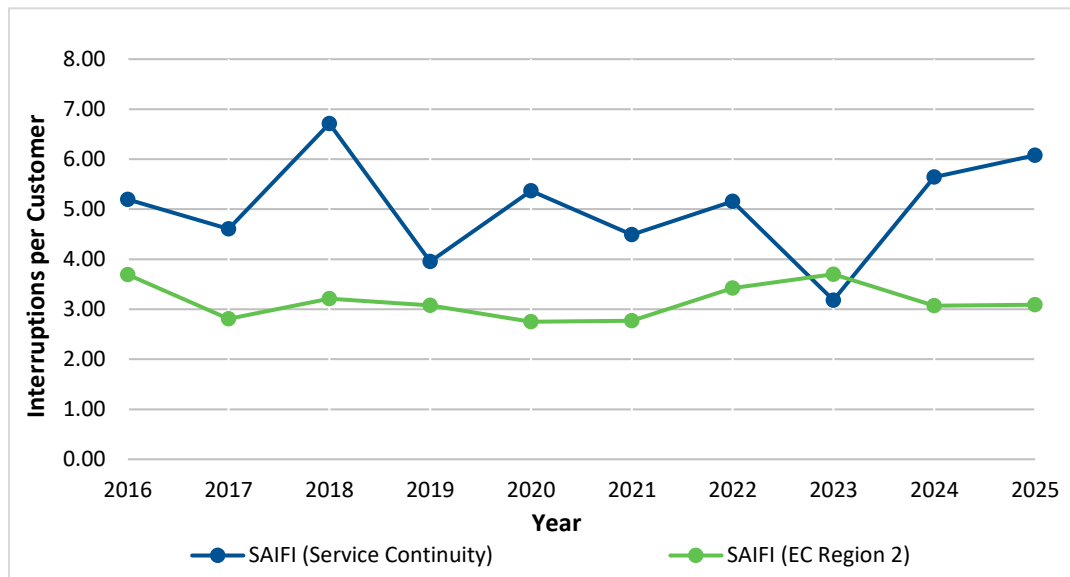
Chart 1: SAIFI Excluding Major Events – Central
