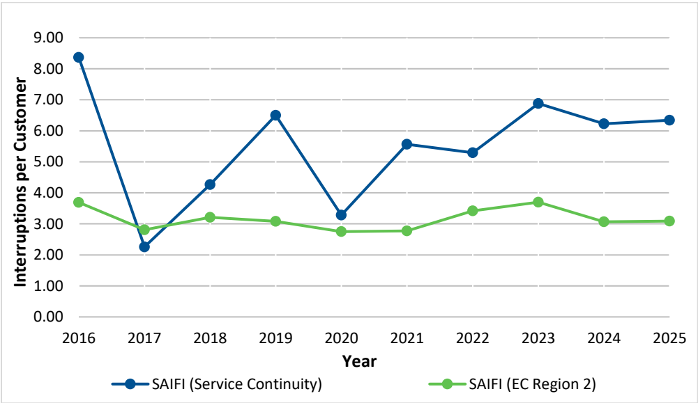
Chart 6: SAIFI Including Major Events – Northern
