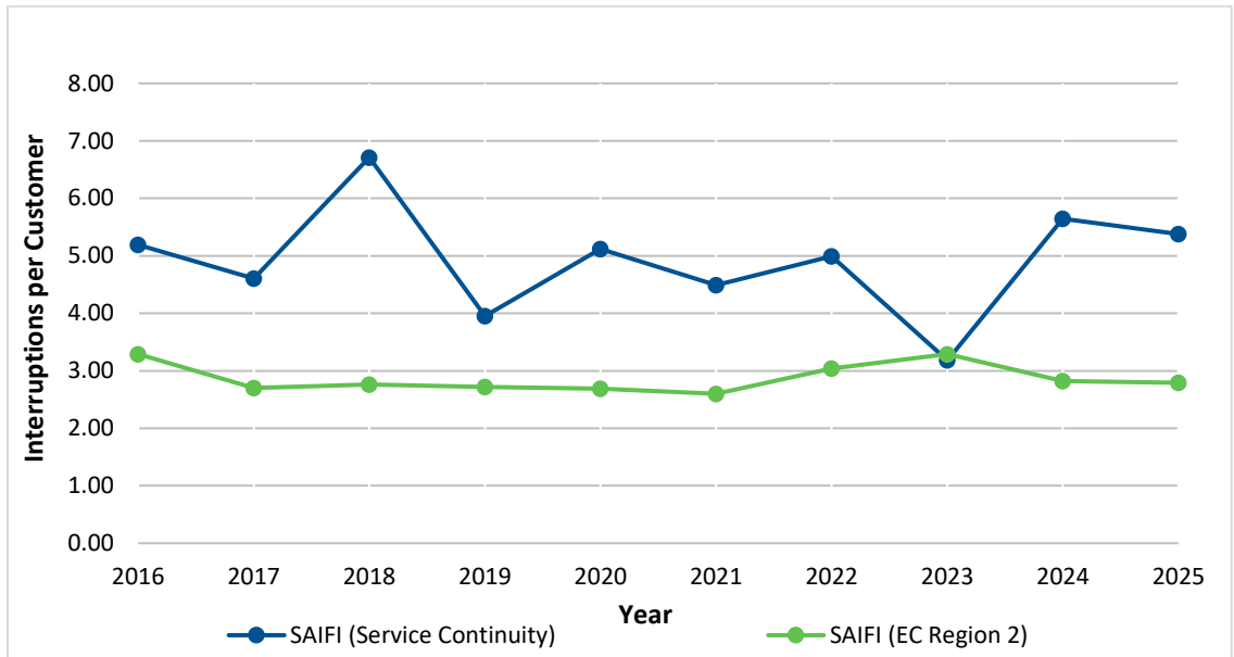
Chart 1: SAIFI Excluding Major Events – Central
