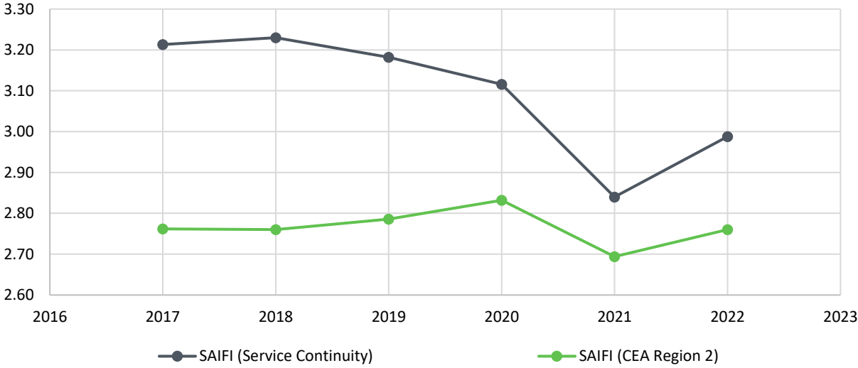
Chart 6: SAIFI Excluding Major Events – Island
