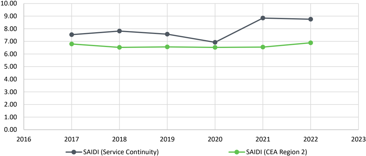
Chart 12: SAIDI Excluding Major Events – Labrador
