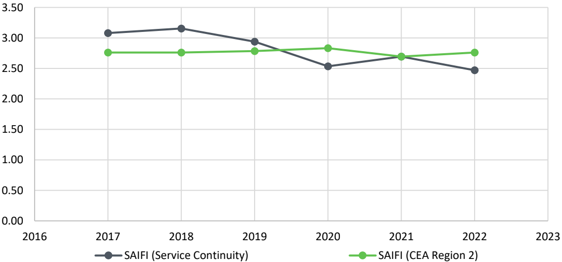
Chart 10: SAIFI Excluding Major Events – Labrador
