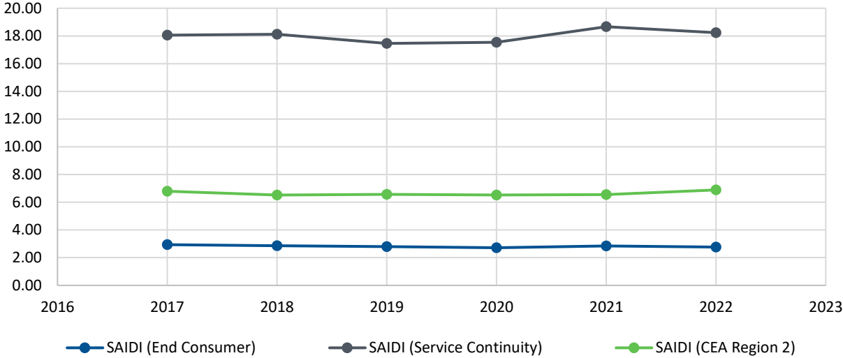
Chart 4: SAIDI Excluding Major Events - Hydro System
