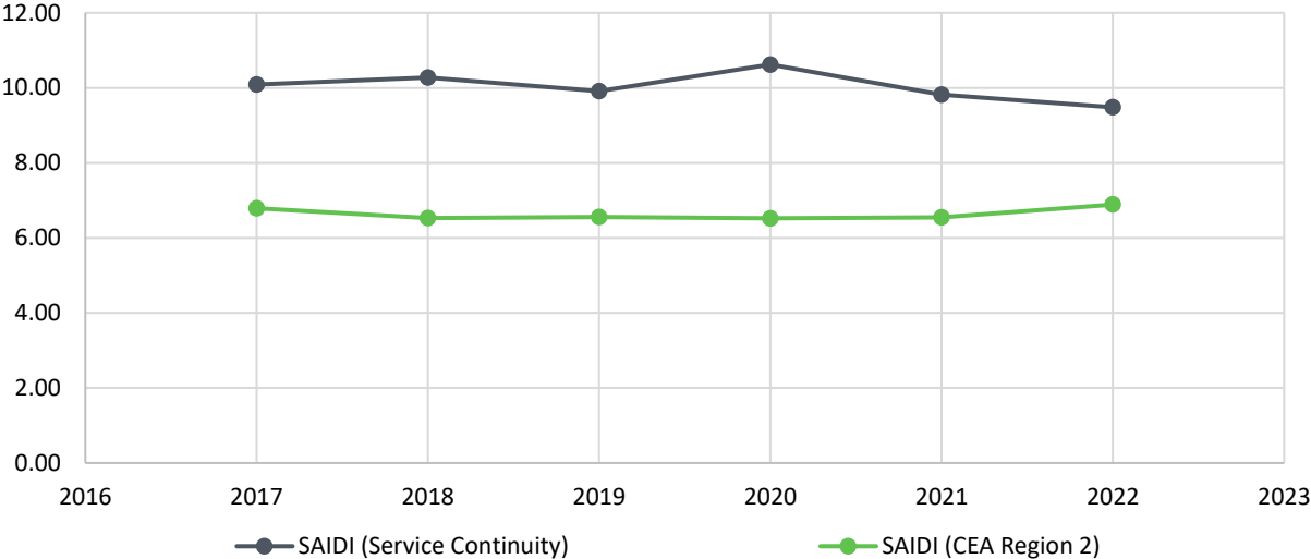
Chart 8: SAIDI Excluding Major Events – Island
