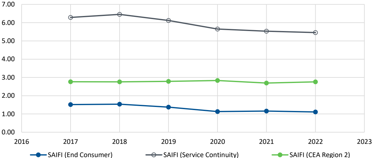
Chart 2: SAIFI Excluding Major Events – Hydro System
