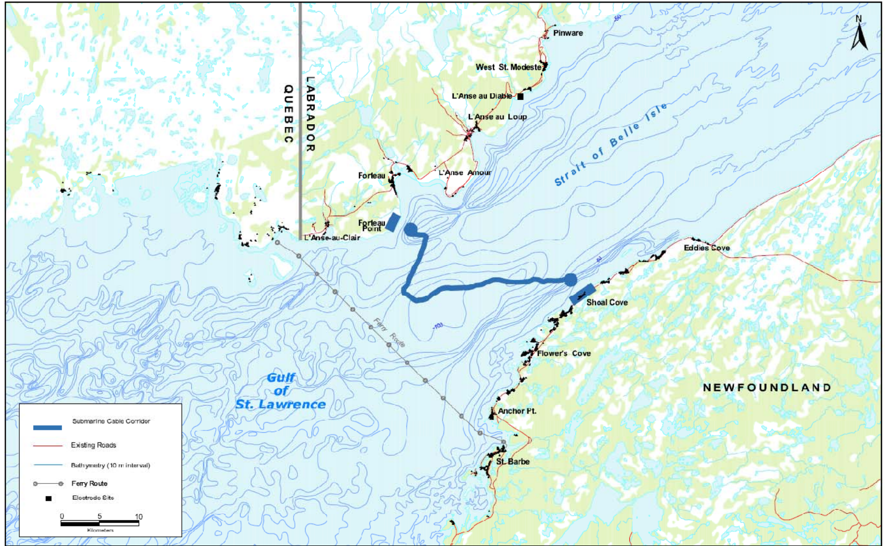
Figure 1.1-1: Study Area and Strait of Belle Isle Submarine Cable Crossing Corridor.
