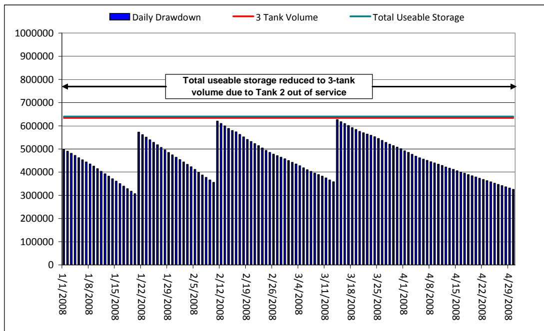
Holyrood Fuel Storage Levels 2008
