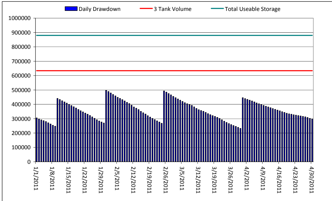
Holyrood Fuel Storage Levels 2011
