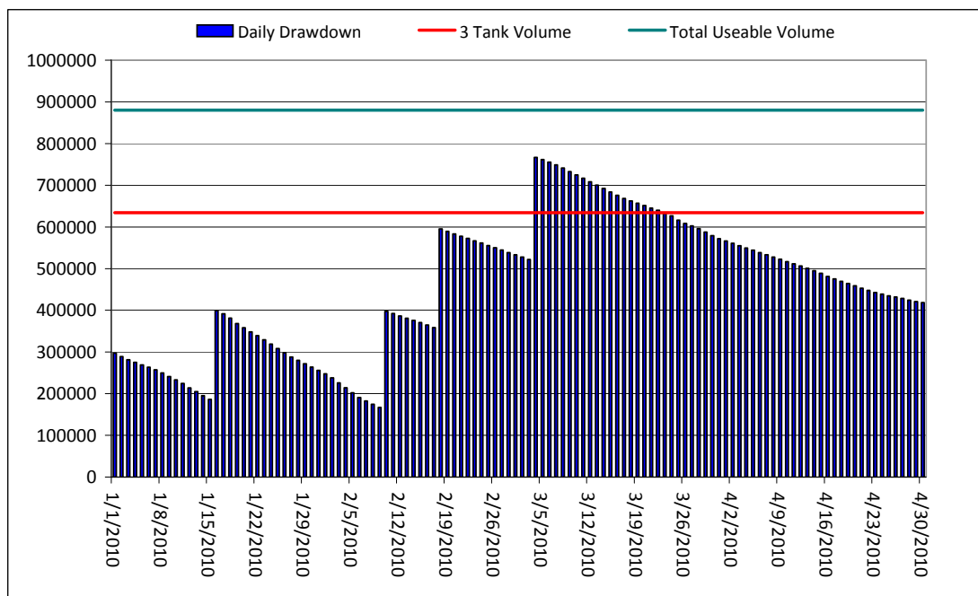
Holyrood Fuel Storage Levels 2010
