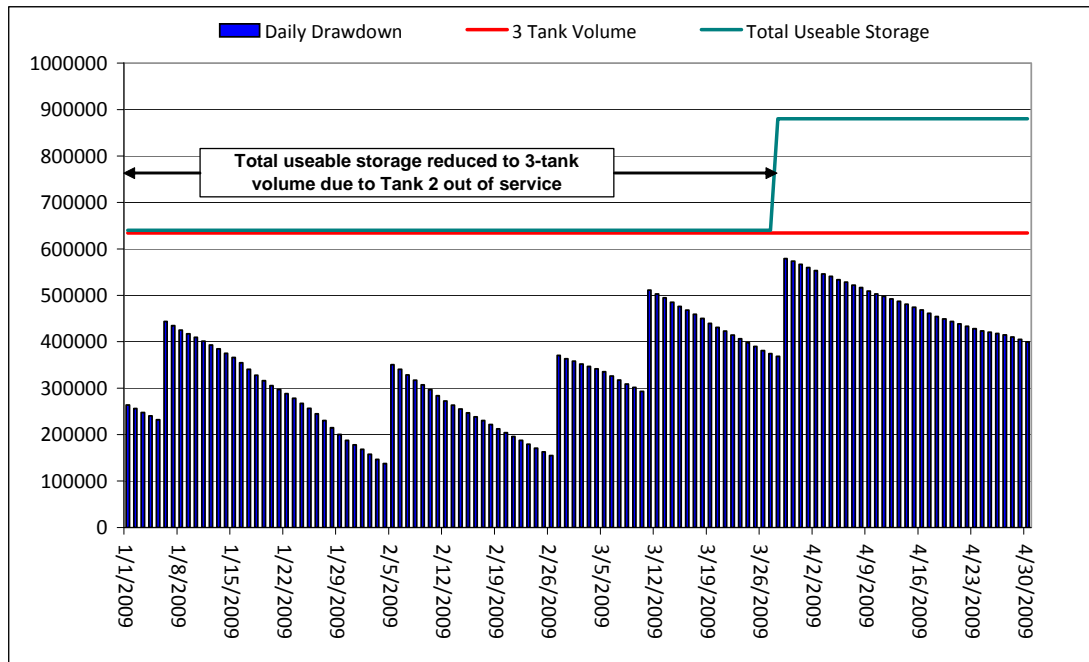
Holyrood Fuel Storage Levels 2009
