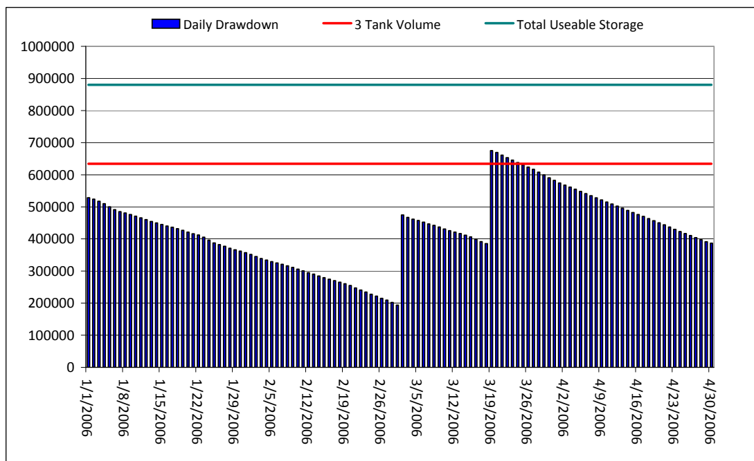
Holyrood Fuel Storage Levels 2006
