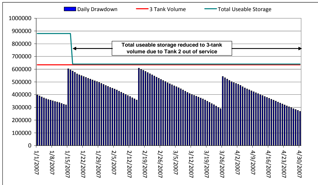
Holyrood Fuel Storage Levels 2007
