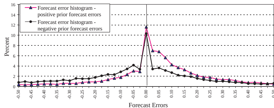
Fig. 3. Histogram of forecast errors by sign of prior abnormal returns (Panel A), prior earnings changes (Panel B), and prior forecast errors (Panel C). This figure presents the percentage of forecast error values in histogram intervals for observations within forecast error of -0.5 to +0.5 by sign of prior abnormal return (Panel A), prior earnings changes (Panel B), and prior forecast errors (Panel C). Forecast error is reported earnings minus the last consensus forecast of quarterly earnings issued prior to earnings announcement scaled by the beginning-of-period price. Prior abnormal return is the return between 10 days after the last quarterly earnings announcement to 10 days prior to current quarterly earnings announcement minus the return on the value-weighted market portfolio for the same period. Prior earnings changes are defined as the prior quarter seasonal earnings change (from quarter t - 5 to quarter t - 1 ) scaled by the beginning-of-period price.
