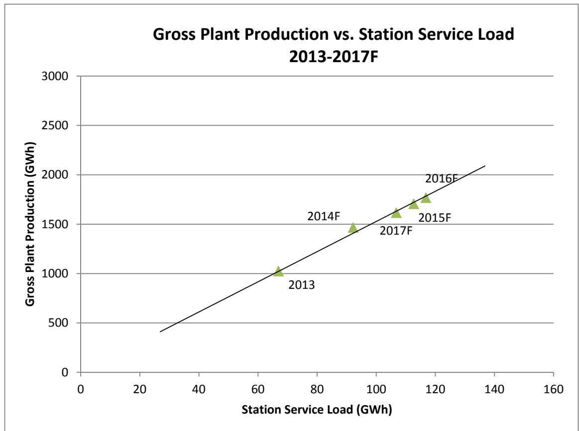
Figure 1: Station Service Load vs Gross Plant Production
