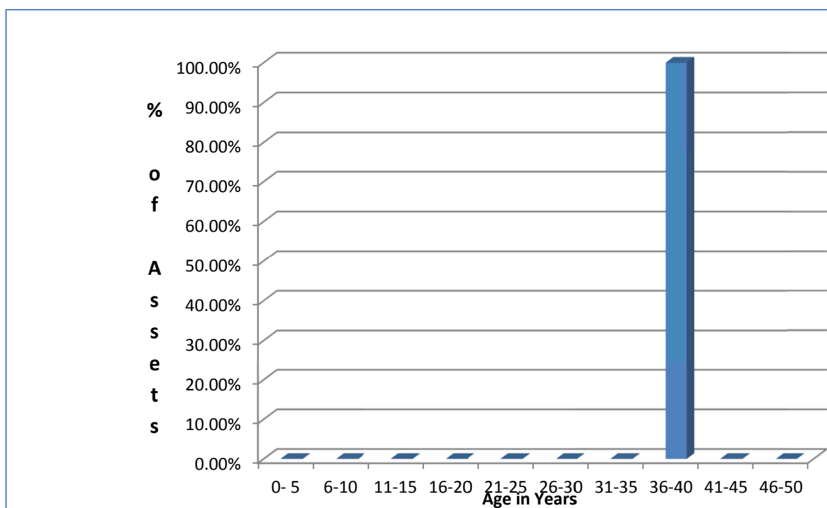
Chart 1: Age Distribution of Transmission Assets – Labrador Interconnected System
