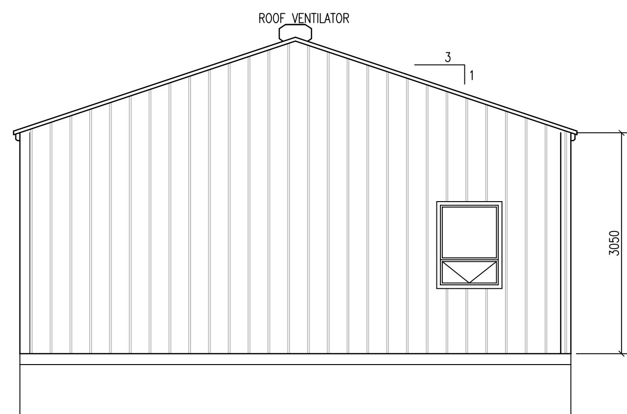
SIDE ELEVATION
