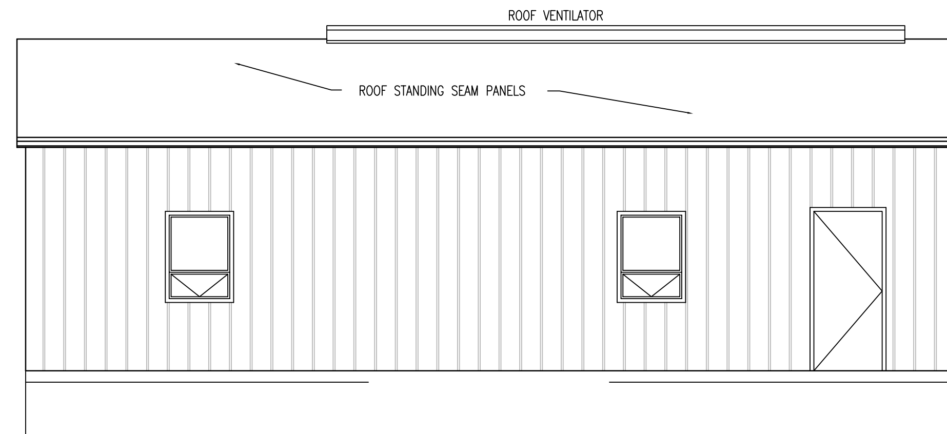
REAR ELEVATION
