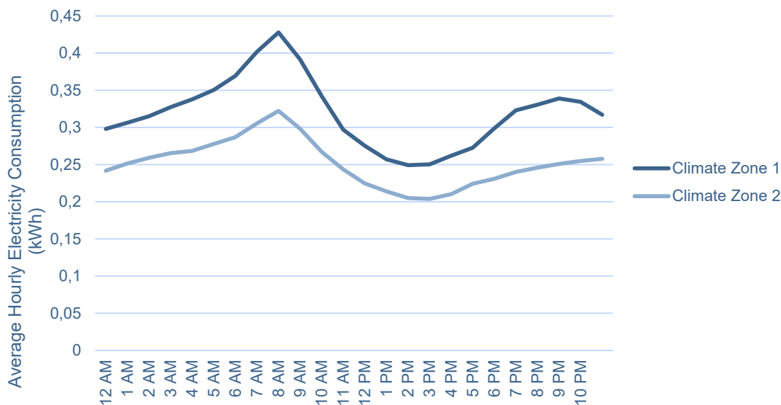
Figure 12: DHP Average Electricity Consumption in October
