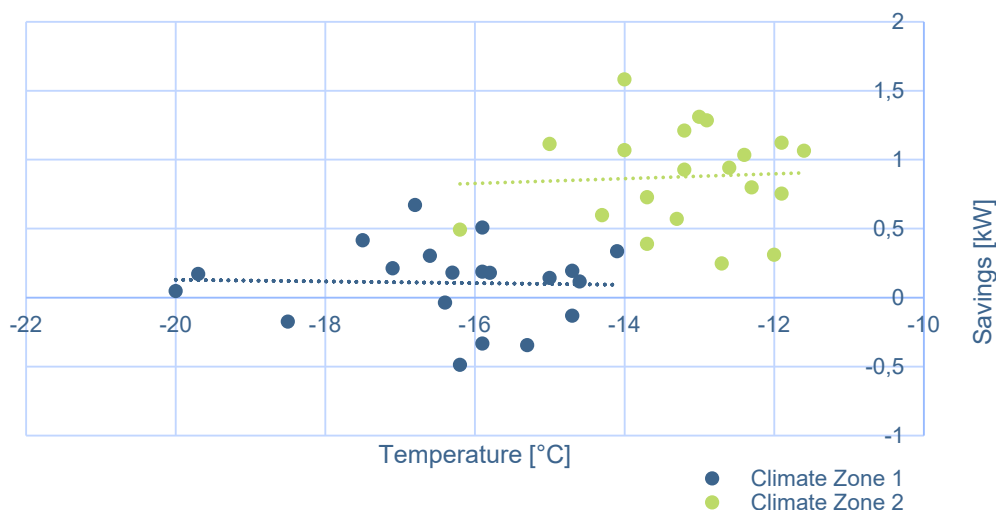
Figure 7: Demand Savings as a Function of Outside Temperature During Top-20 Peak Hours
