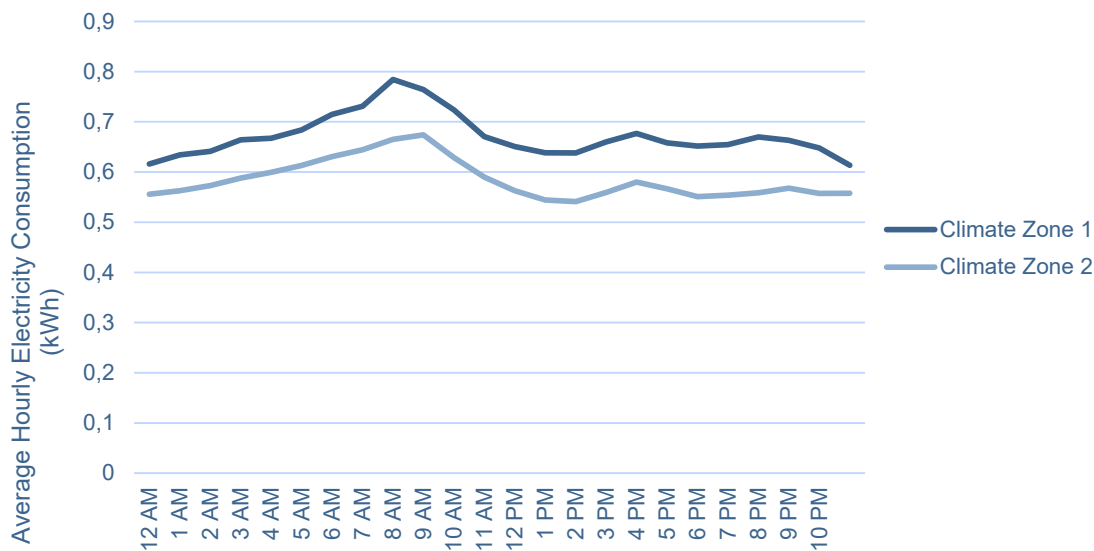
Figure 13: DHP Average Electricity Consumption in December
