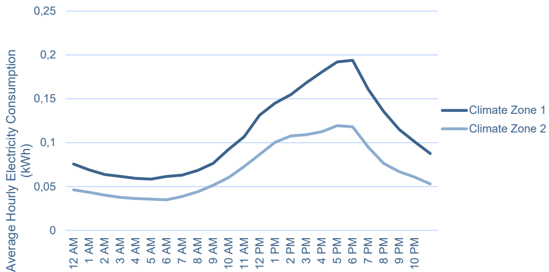
Figure 11: DHP Average Electricity Consumption in August
