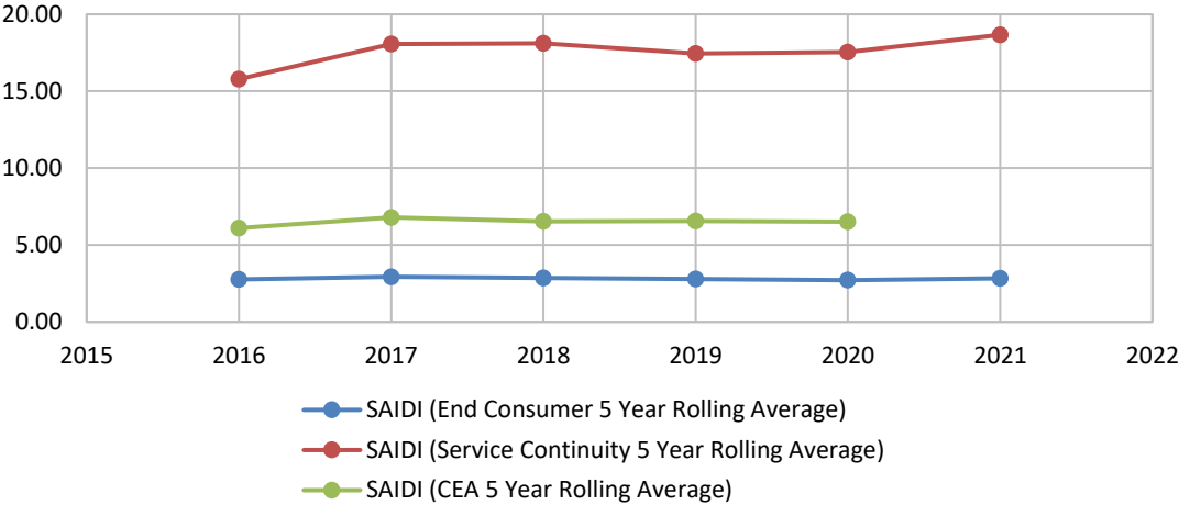
Chart 1: SAIDI Excluding Significant Events
