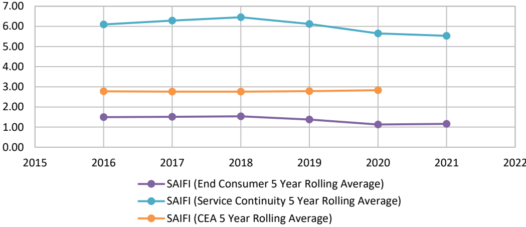
Chart 2: SAIFI Excluding Significant Events
