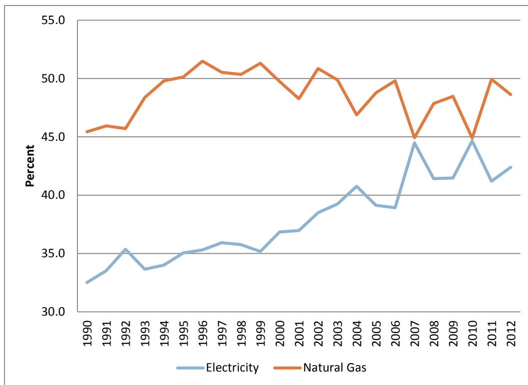
1 Figure 10: Residential Energy Use for British Columbia 2 Natural Gas v. Electricity 1990 – 2012
